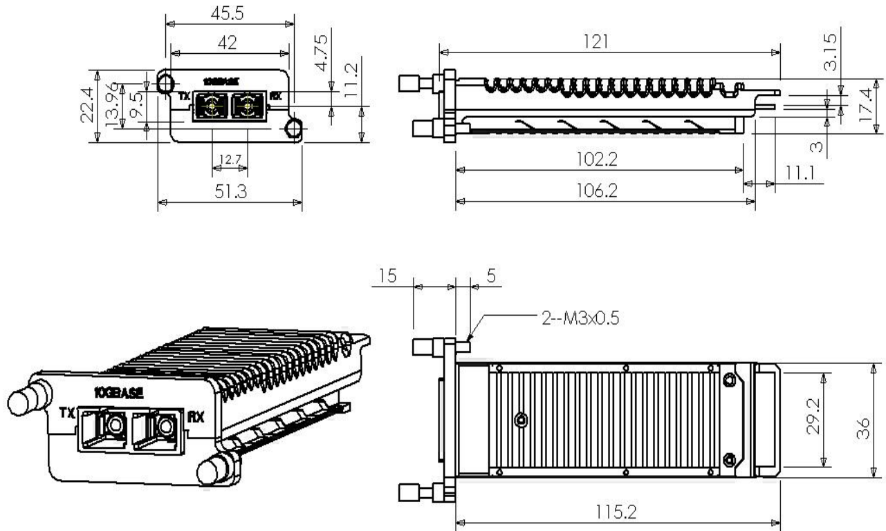
Figure 1 Mechanical dimensions
